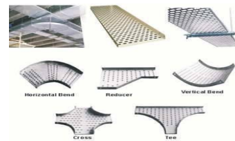
Cable Tray Accessories
